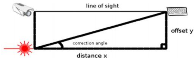
Fig. 10. The angle of correction when the laser and the camera have offset between them
