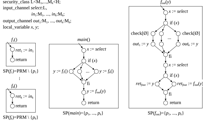
Fig. 7. Program \pi_b(k) .
