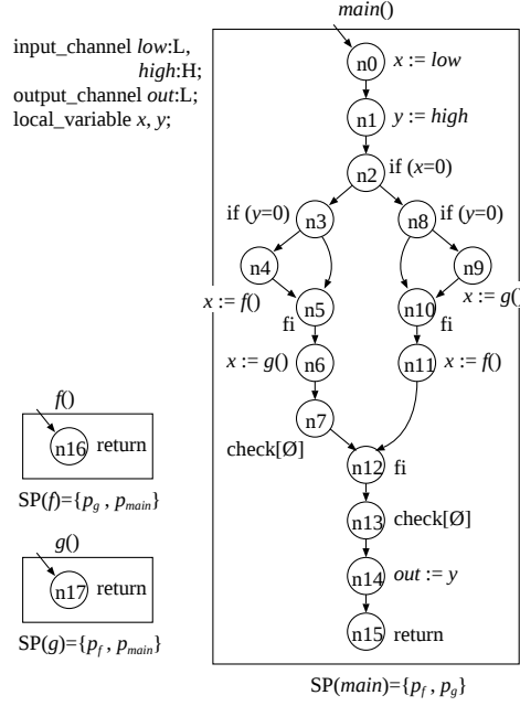
Fig. 4. Program \pi_2 .
