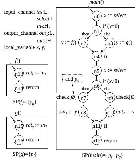
Fig. 3. Program \pi_1 .
