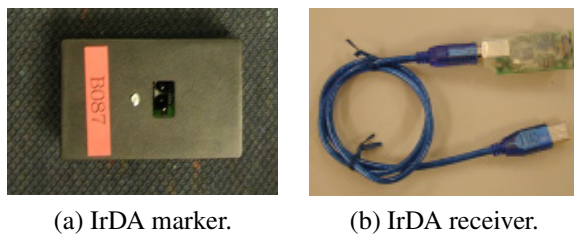
Figure 2. IrDA sensors.
