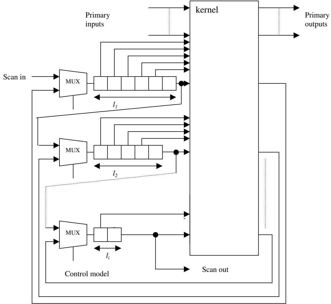
Figure 5. FSR scan designed circuit.
