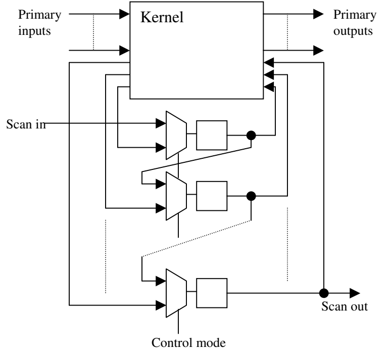
Figure 3. Scan designed circuit
