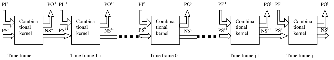
Figure 6. Iterative logic array model.
