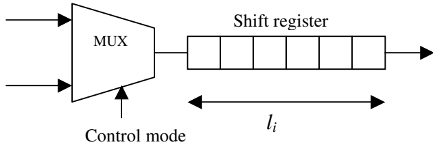
Figure 4. Scan shift register.
