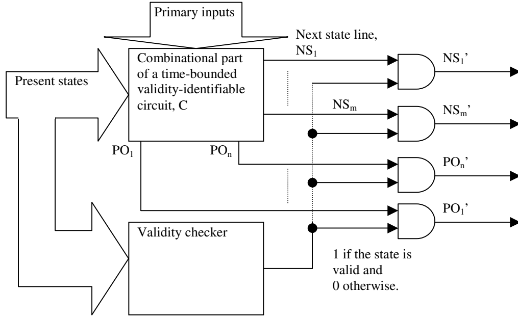
Figure 7. Transformed combinational part C' of a time-bounded validity-identifiable circuit.
