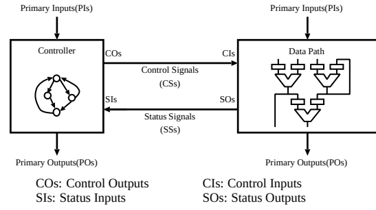
Figure 1: An RTL controller/data path circuit.
