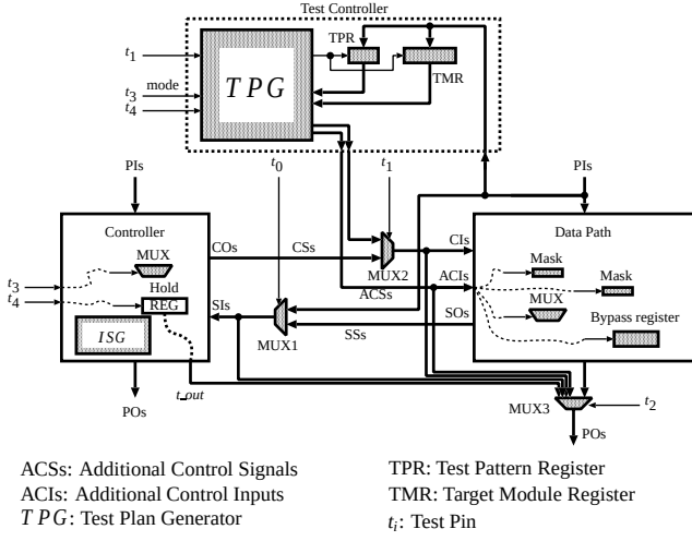
Figure 2: Test architecture of a controller/data path circuit.
