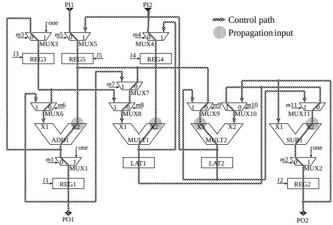
Figure 6: An example of a control forest.
