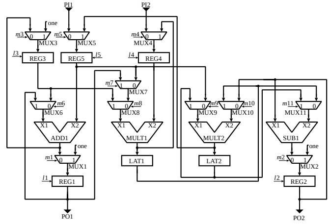
Figure 5: An example of a data path.
