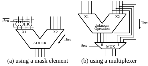
Figure 4: Examples of realizing thru function.
