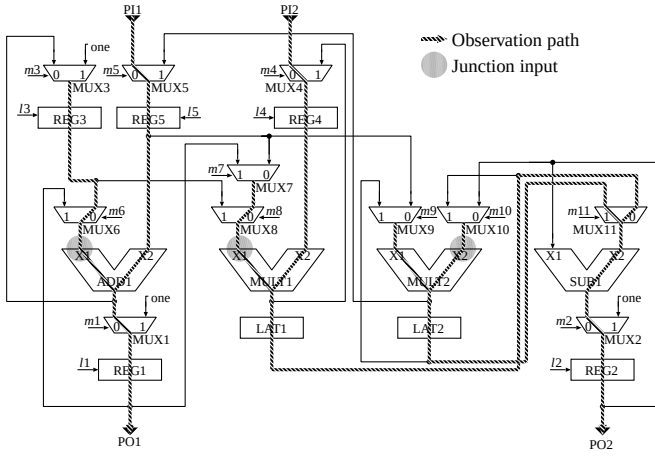
Figure 7: An example of an observation forest.
