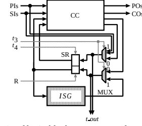
Figure 3: A controller augmented with an extra logic ISG.
