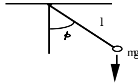
Figure 2 A simple pendulum where the particle with mass m is suspended by a string
