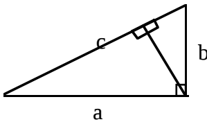
Figure 1 Geometric object for Pythagorean theorem
