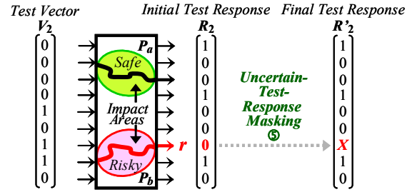
Figure 7. Uncertain-test-response masking.
